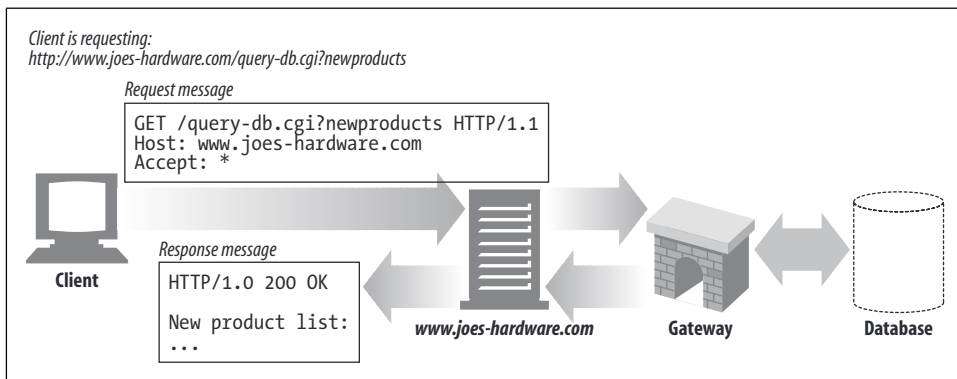
Figure 8-1. Gateway magic
