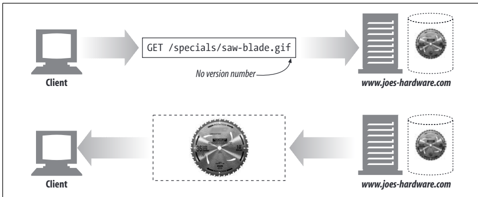
Figure 3-6. HTTP/0.9 transaction
