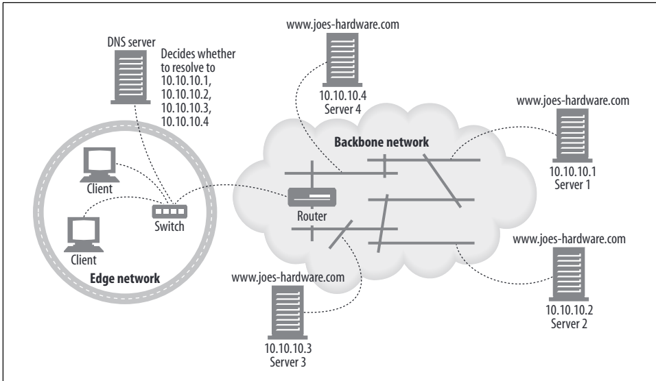
Figure 20-2. DNS-based redirection
