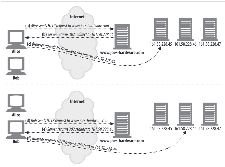
Figure 20-1. HTTP redirection
