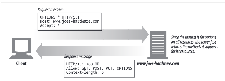
Figure 3-12. OPTIONS example
