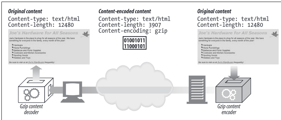
Figure 15-3. Content-encoding example
