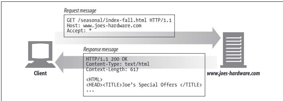
Figure 3-7. GET example
