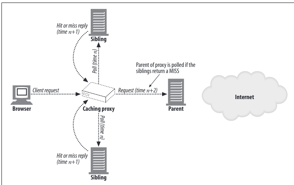
Figure 20-13. ICP queries
