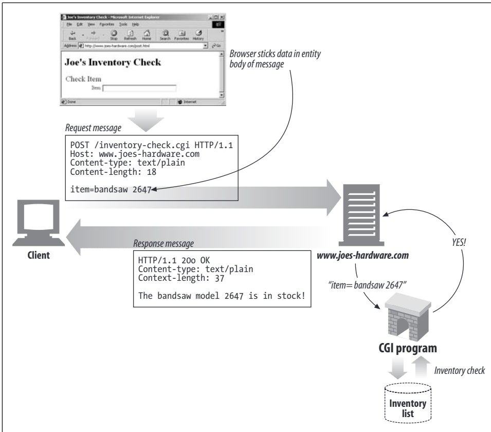
Figure 3-10. POST example
