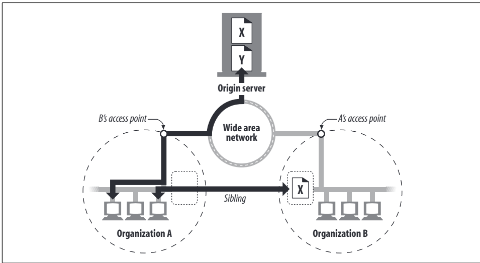
Figure 7-10. Sibling caches
