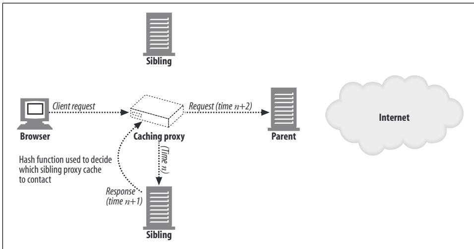
Figure 20-14. CARP redirection
