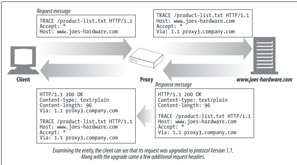
Figure 3-11. TRACE example
