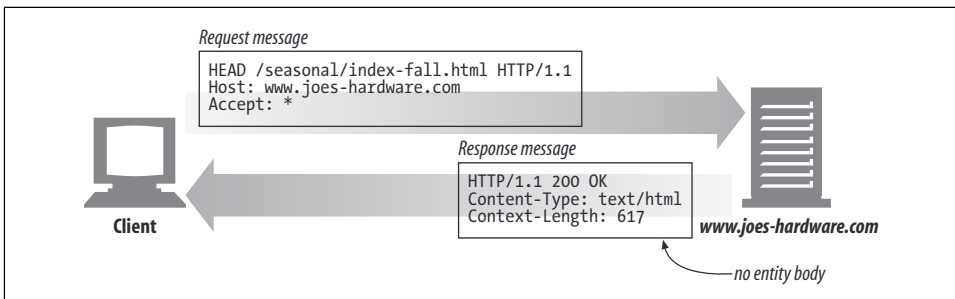
Figure 3-8. HEAD example
