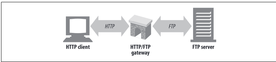
Figure 1-13. HTTP/FTP gateway
