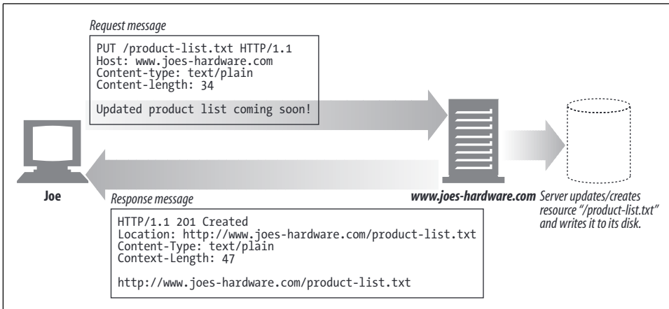
Figure 3-9. PUT example
