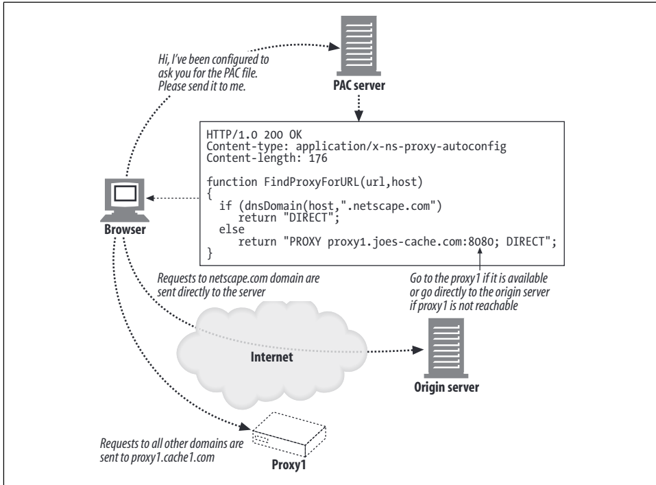
Figure 20-10. Proxy auto-configuration
