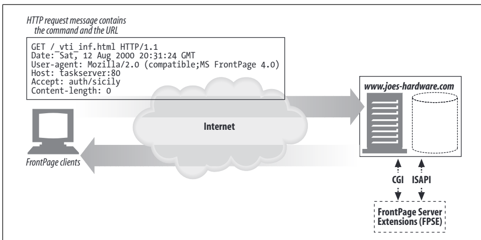
Figure 19-2. Initial request
