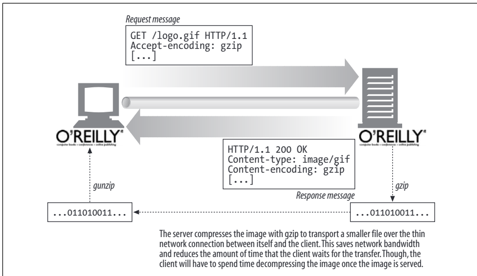
Figure 15-4. Content encoding
