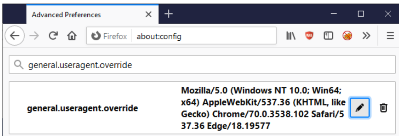
Figure 6.F-2: Mozilla Firefox User-Agent Switching Functionality
