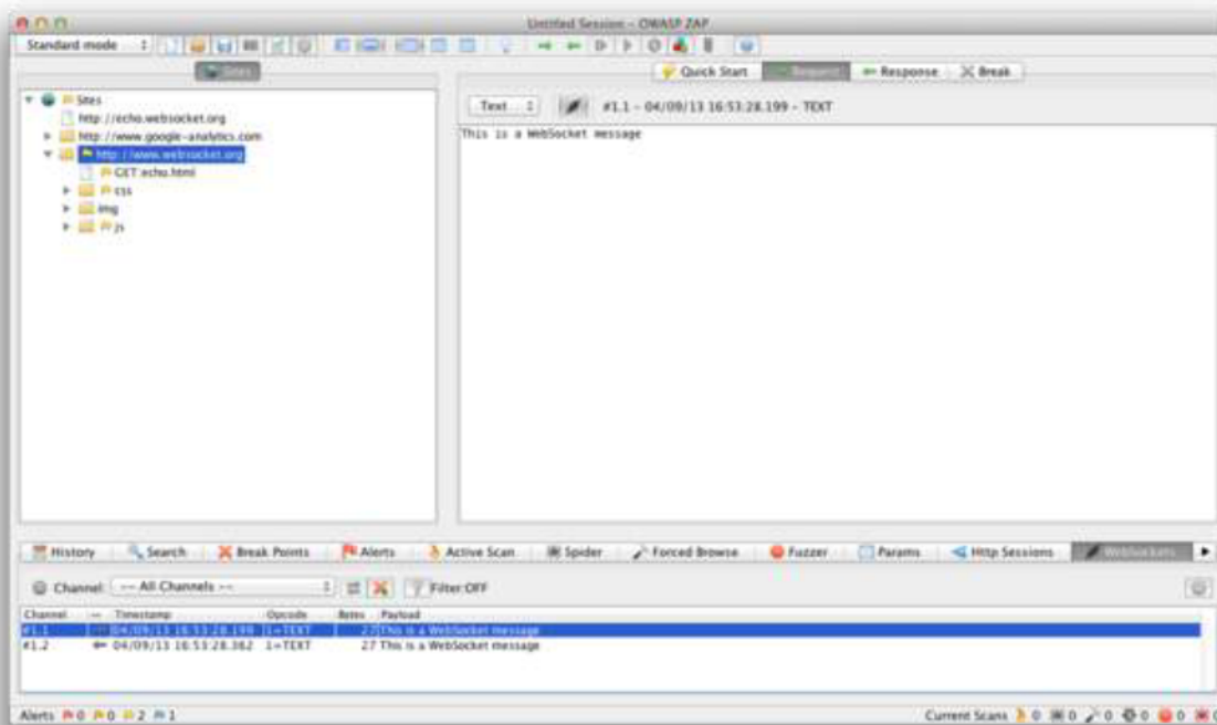
Figure 4.11.10-1: ZAP WebSockets
