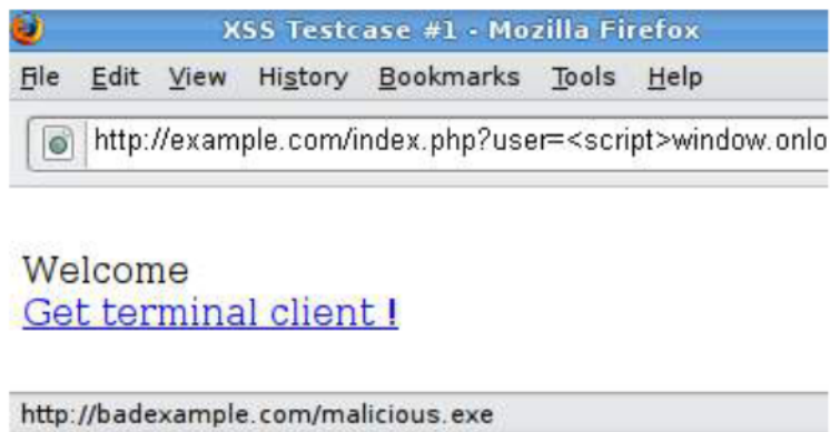
Figure 4.7.1-3: XSS Example 2
